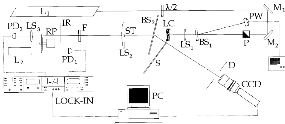
Figure 1. The experimental set-up.
