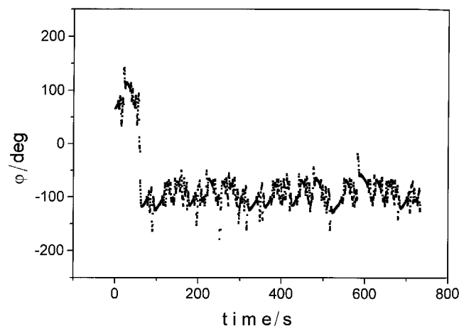
Figure 10. Azimuthal angle \phi of \mathbf{n} as a function of time, showing chaotic motion. I = 3.75I_{th} .
